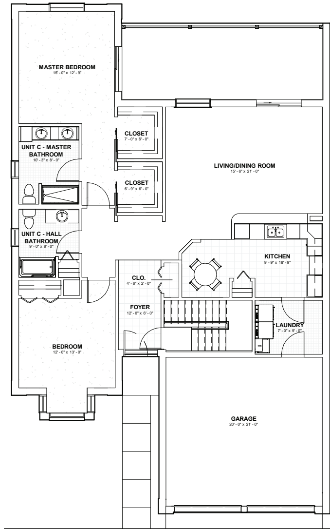
FLOOR PLAN
